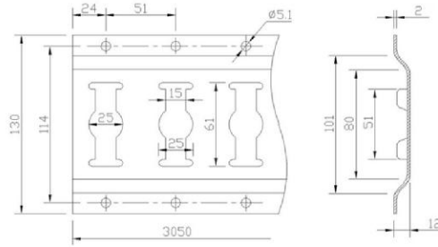
F14010 Zinc plated
