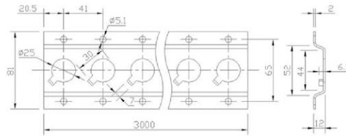
F14020 Zinc plated
