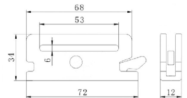
F14503 Zinc plated
